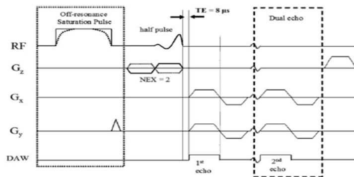
Figure 4. Pulse sequence
