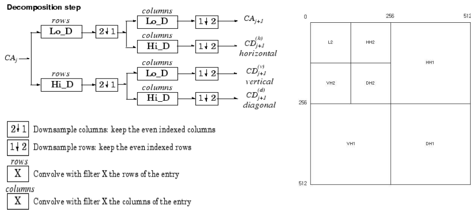
Figure 2. Decomposition and synthesis of two-dimensional signals by DWT
